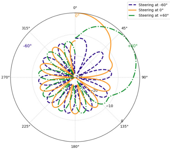
Fig. 8: Simulated radiation patterns at -60^\circ , 0^\circ , and +60^\circ steering angles.
